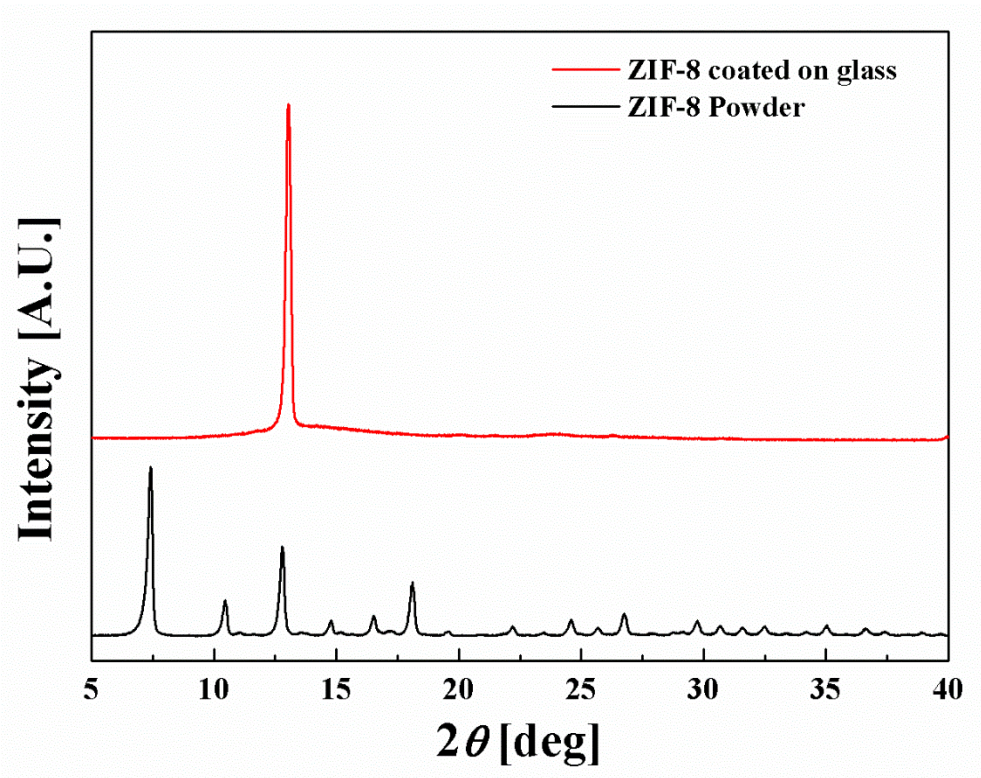
Figure S2. XRD pattern of ZIF-8 coated on glass with DMF in solution
