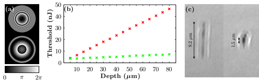
Fig. 3. (a) Phase pattern displayed on the SLM with (top) and without (bottom) inclusion of the defocus. (b) Plot of the measured fabrication threshold energy for the uncompensated (red) and compensated (green) cases. (c) Side views of fabricated voxels at a depth of 20\ \mu\text{m} when the beam is uncompensated (left) and compensated (right).
