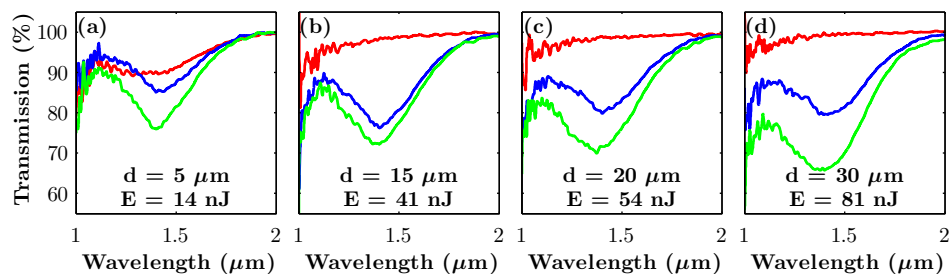
Fig. 5. Smoothed transmission spectrum of FCC PhCs of 16 layers and a lattice constant of 4.5 \mu\text{m} fabricated with a depth below the surface and energy above fabrication threshold of (a) 5 \mu\text{m} and 14 nJ, (b) 15 \mu\text{m} and 41 nJ, (c) 20 \mu\text{m} and 54 nJ, (d) 30 \mu\text{m} and 81 nJ. The red spectrum correspond to PhCs with no compensation while the blue and green spectrum correspond to PhCs with aberration compensation based on the isotropic aberration function and our adaptive compensation method, respectively.
