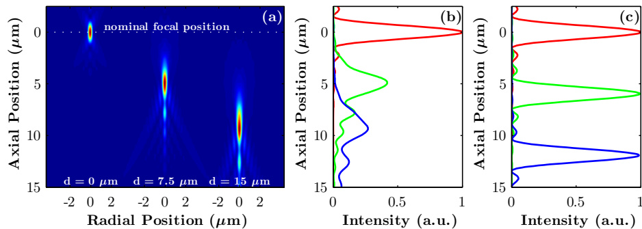
Fig. 1. (a) Calculated focal intensity distribution when a plane wave is focused into depths of 0 \mu\text{m} , 7.5 \mu\text{m} and 15 \mu\text{m} in LiNbO 3 without compensation of the refractive-index mismatch aberration. (b) Comparison of the intensity along the axial direction in (a). (c) Intensity along the axial direction in (a) when the aberration is compensated.
