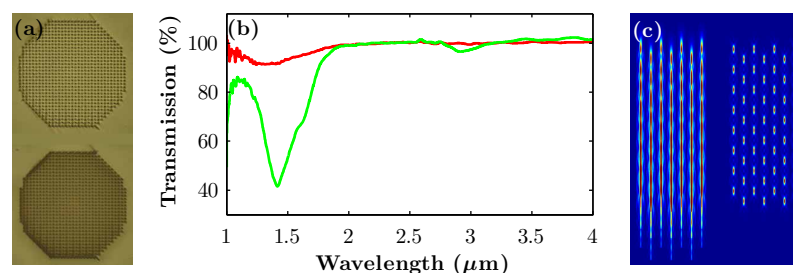
Fig. 4. (a) Transmission microscope images of the top view of FCC PhCs of 50 layers and of lattice constant 4.5 \mu\text{m} fabricated without (top) and with (bottom) compensation of the refractive-index mismatch aberration. (b) Smoothed transmission spectrum of the uncompensated (red) and compensated (green) PhCs in (a). (c) Calculated focal intensity distributions that occur when fabricating the top 16 layers of the uncompensated (left) and compensated (right) PhCs in (a).
